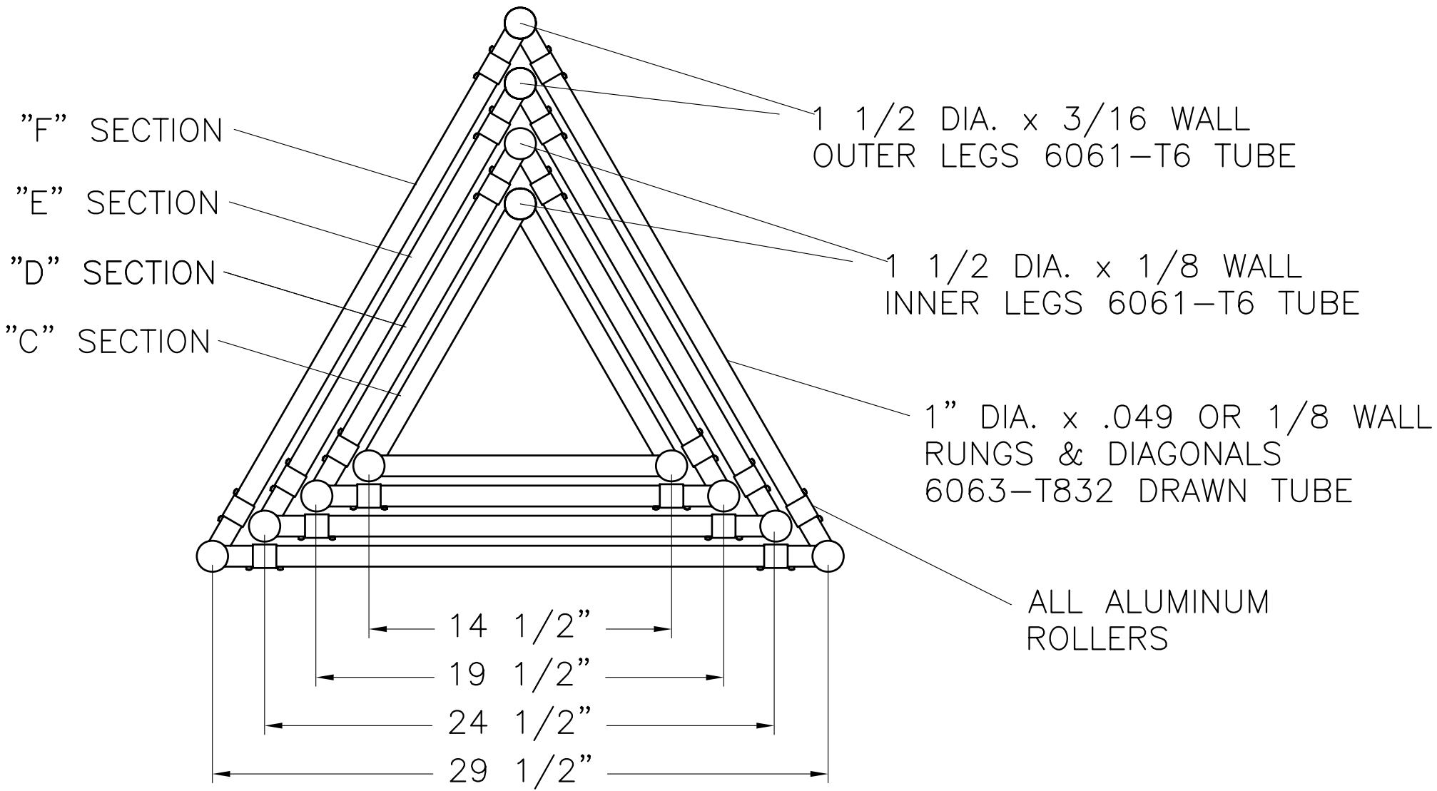
UNGUAYED CROSS SECTION
